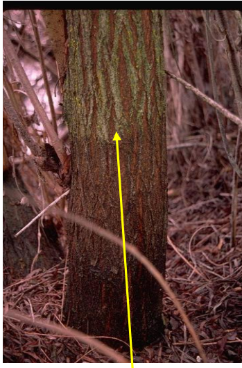
Figure 19: Water mark on tree showing vertical extent of seasonal ponding.
