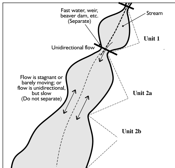
Figure 1. Determining wetland units along a stream corridor with constrictions. Units 2a and 2b should be rated as one unit.
