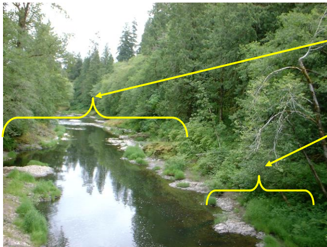
Figure 26. A riverine wetland where the width of the wetland is less than the distance between banks (< 1).
